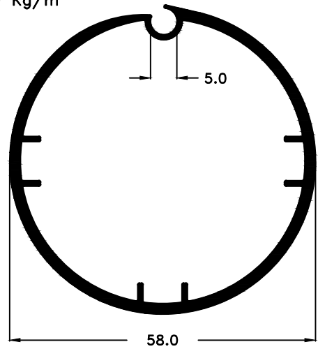
PM-2008 1,000 Kg/m
