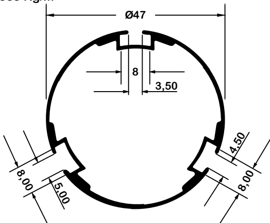
PM - 1952 0,585 Kg/m
