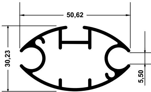
PM-3454 0,792 Kg/m
