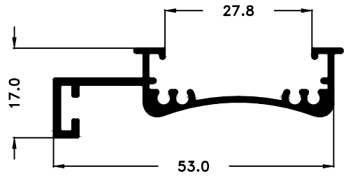
PM-4705 0,399 Kg/m
